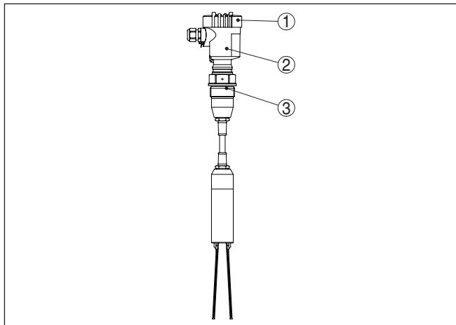
插图. 1: VEGAWAVE 62, 带塑料外壳
