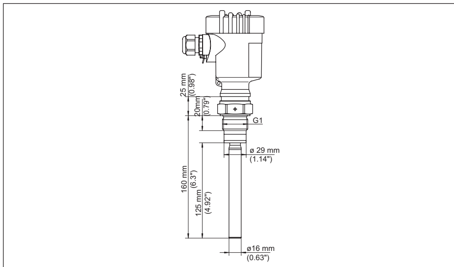
插图. 20: VEGAVIB 61, 螺纹型 G1 (DIN ISO 228/1)
