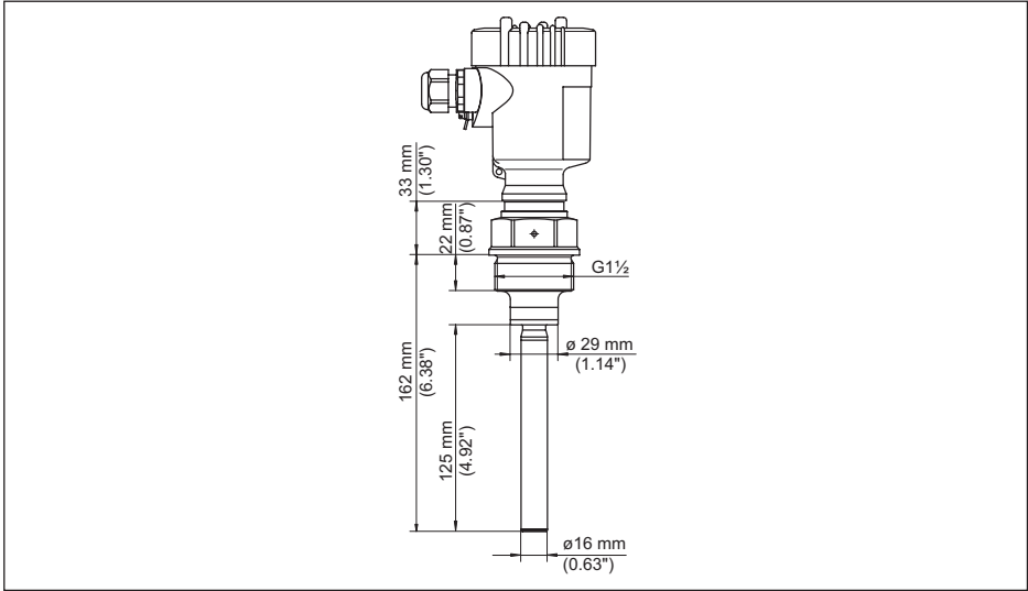
插图. 17: VEGAVIB 61, 螺纹型 G1½ (DIN ISO 228/1)
