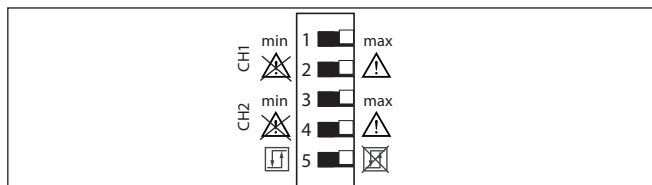
插图. 2: DIL 开关 VEGATOR 112
