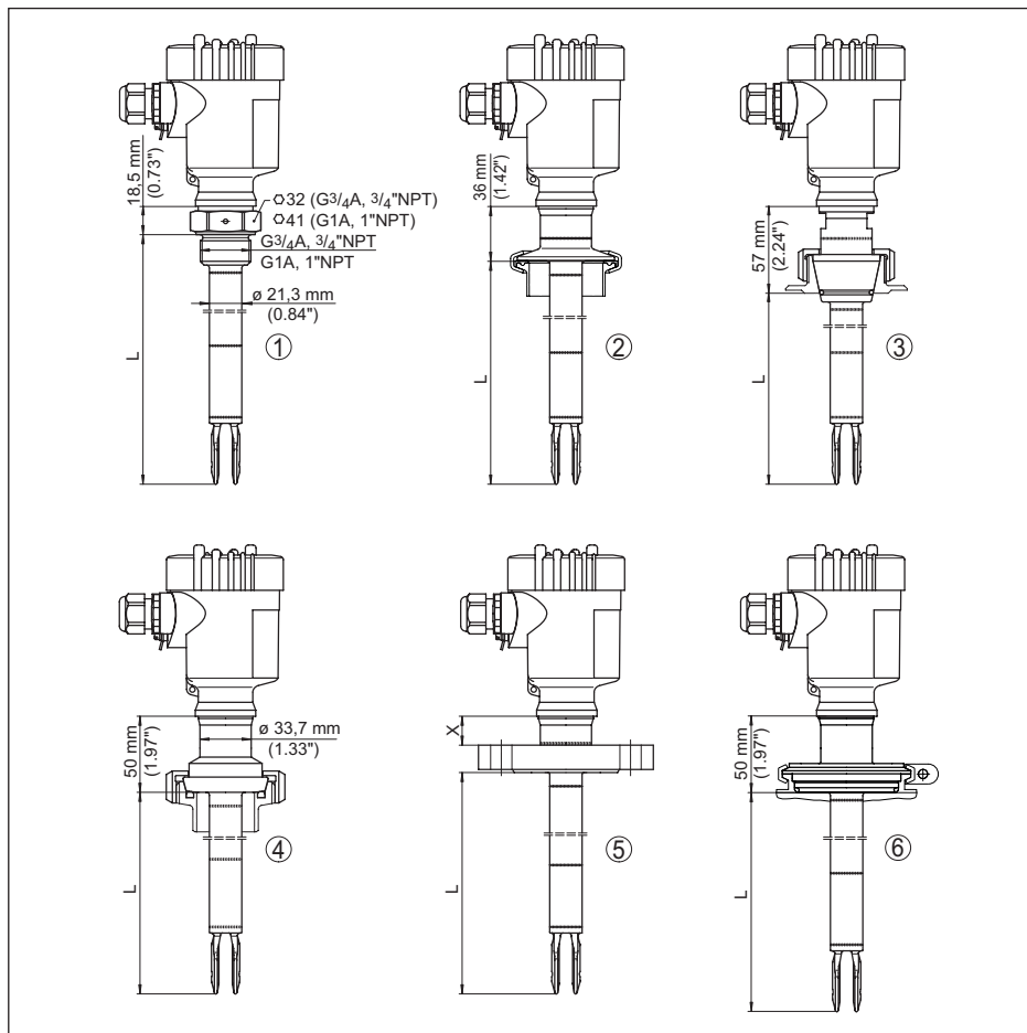
插图. 23: VEGASWING 63
