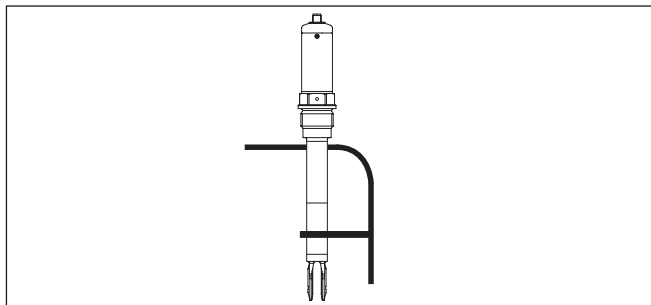
插图. 7: VEGASWING 53 的侧面支撑
