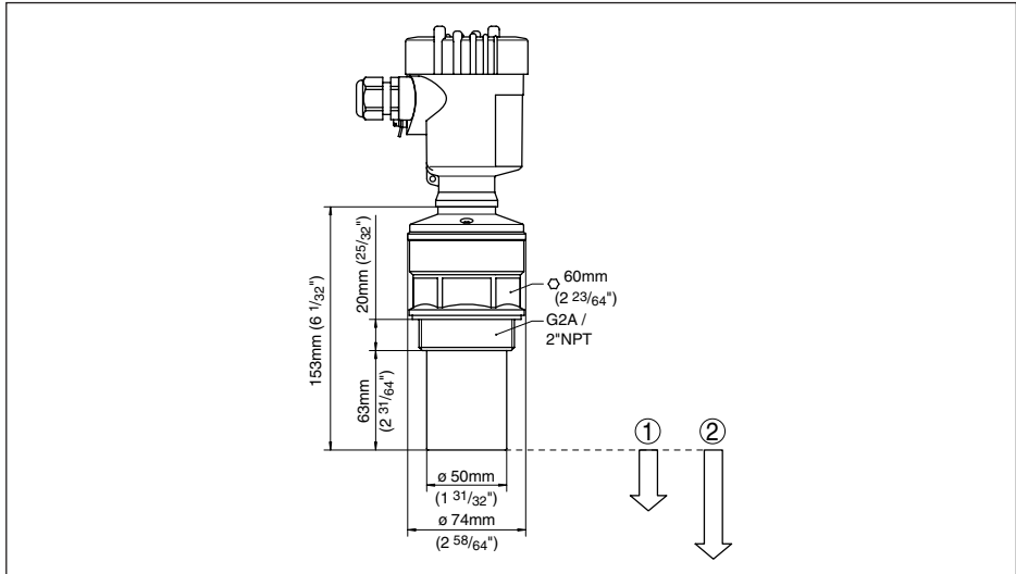
插图. 40: VEGASON 62
