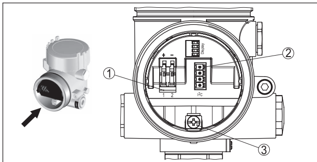
插图. 24: 双腔式外壳的接线腔
