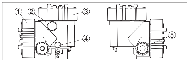
插图. 22: 双腔式外壳
