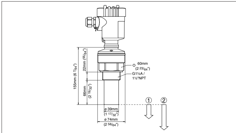
插图. 44: VEGASON 61
