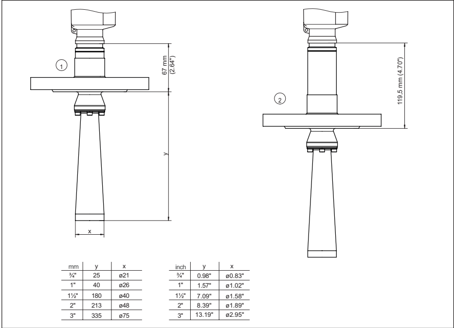
插图. 103: VEGAPULS 6X, 带有喇叭口天线的法兰，至 +150 °C (+302 °F)/+250 °C (+482 °F)
