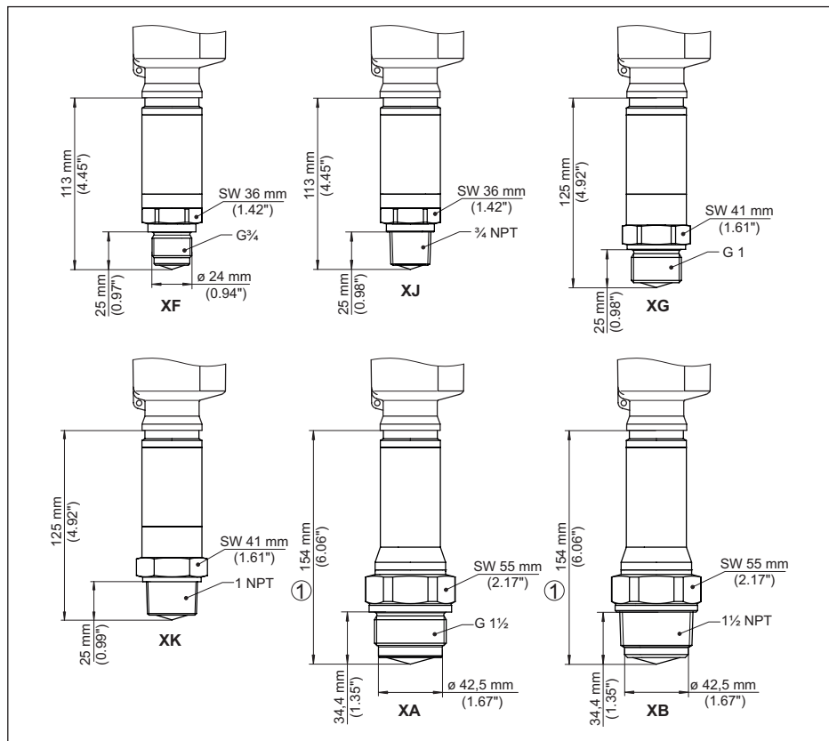
插图. 102: VEGAPULS 6X, 带有内置天线系统的螺纹至 +200 °C (+392 °F)/+250 °C (+482 °F)
