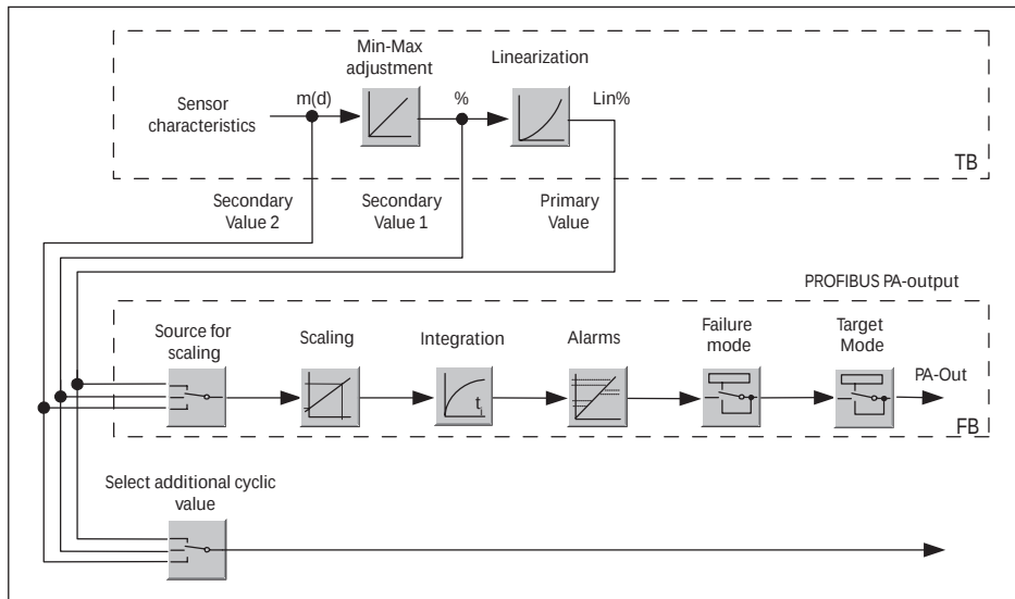
插图 33: VEGAPULS 67: Block diagram with AI (PA-OUT) value and additional cyclical value
