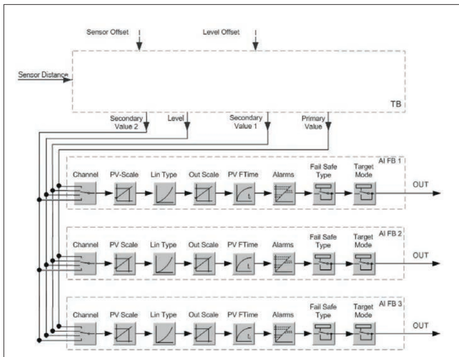
插图. 46: VEGAPULS 65: Block diagram with AI FB 1 ... AI FB 3 OUT values
