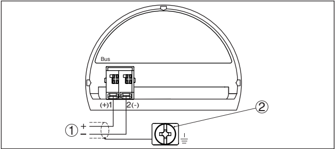
插图. 16: 防爆 (Ex-d-ia) 型双腔式壳体的接线腔
