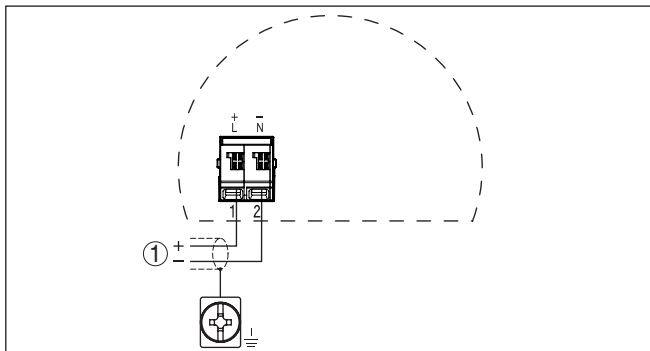
插图. 7: 发射单元的接线图 - VEGAMIP 61 (Transmitter)
