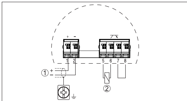
插图. 22: 接收单元的接线图 - VEGAMIP 61 (Receiver) - NPN 表现
