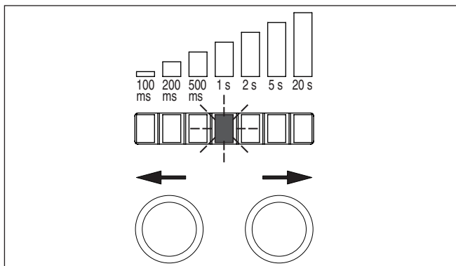
插图. 28: 设置开关延迟 - LED 闪显
