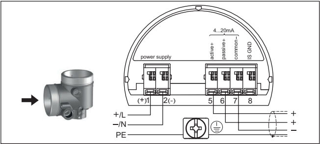
插图. 11: 电网供电时双腔式外壳的接线腔
