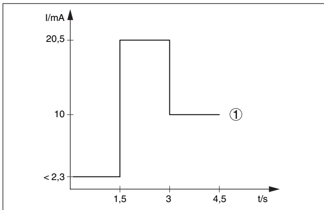
插图. 11: 启动表现
