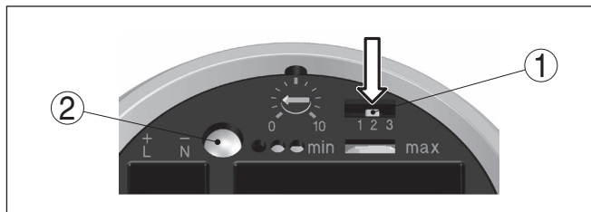
插图. 15: 补偿键
