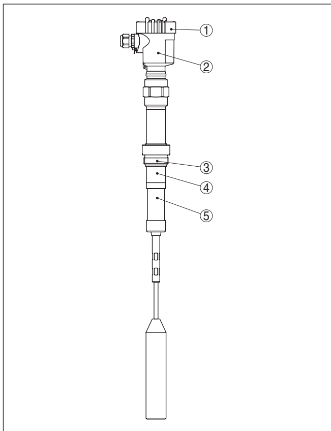
插图. 1: VEGACAP 67, 带塑料外壳
