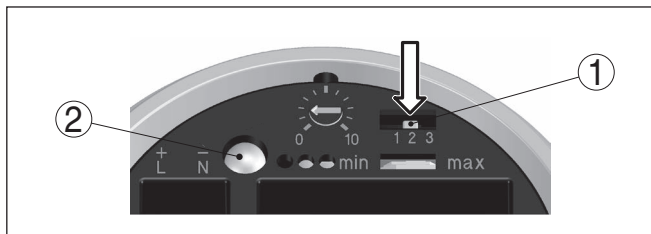
插图. 18: 补偿键
