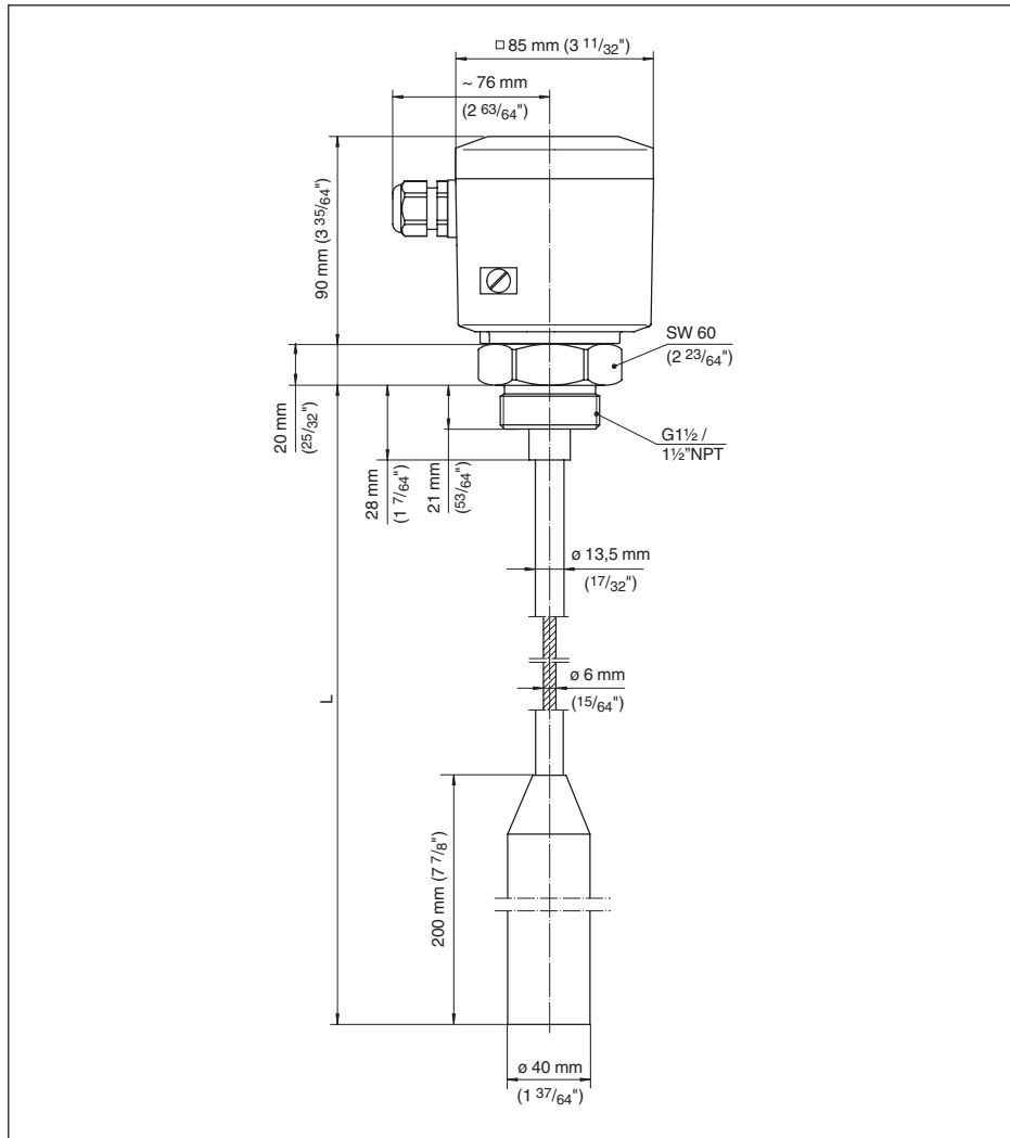
插图. 14: VEGACAP 35, \phi 6 \text{ mm} 绳型, 螺纹型 G1\frac{1}{2} (ISO 228 T1)
