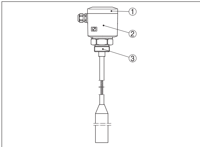
插图. 1: VEGACAP 35
