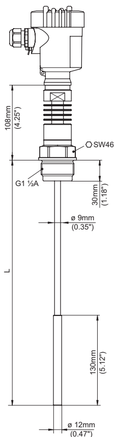
插图. 22: VEGACAL 65, PTFE 绝缘绳 (ø 8 mm) 带压接管 / -50 ... +200 °C
