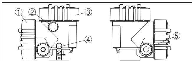
插图. 16: 双腔式外壳
