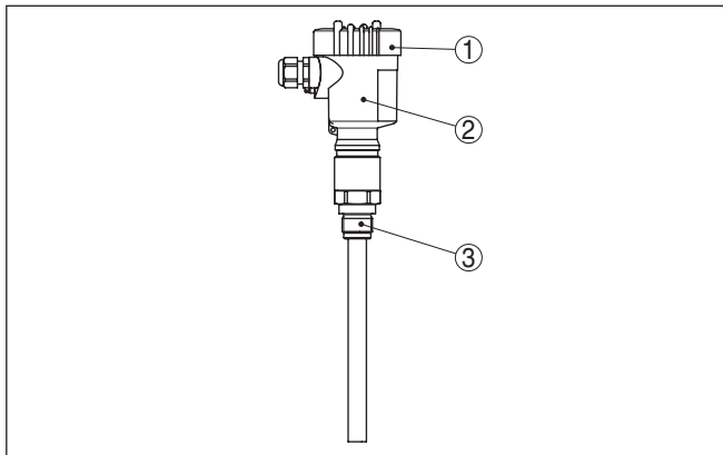
插图. 1: VEGACAL 63, 棒型, 带塑料外壳
