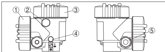
插图. 12: 双腔式外壳
