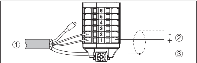
插图. 9: 接线图 VEGABOX 03, 用于 VEGAWELL 52, 4 ... 20 mA, 4 ... 20 mA/HART
