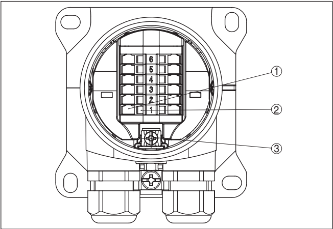
插图. 8: VEGABOX 03 接线腔
