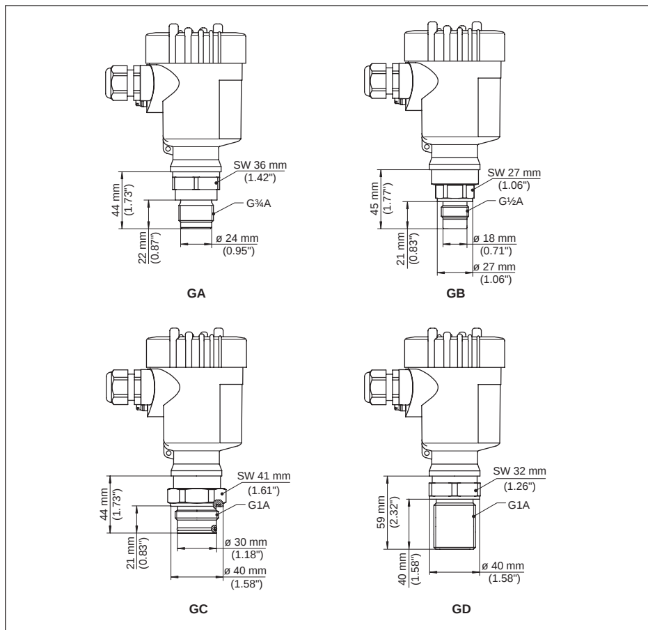
插图. 29: VEGABAR 54, 螺纹接头 : GA = G \frac{3}{4} A 符合 DIN 3852-E, GB = G \frac{1}{2} A 与前壁齐平, GC = G1 A 绝对与前壁齐平, GD = G1 A (DIN 3852-E) x 40 mm 绝对与前壁齐平
