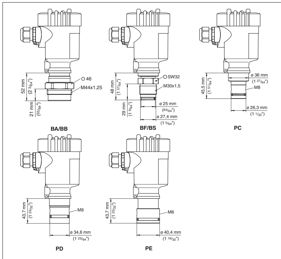
插图. 34: VEGABAR 54, 用于造纸工业的连接 : BA/BB = M44 x 1.25; BF = M30 x 1.5; BS = M30 x 1.5 用于造纸机, PC = PMC 1", PD = PMC 1 1/4", PE = PMC 1 1/2"
