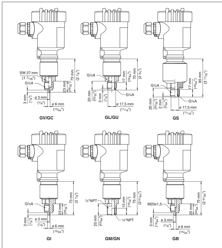
插图. 42: VEGABAR 52, 螺纹接头 : GV/GC = G\frac{1}{2}A 压力计接头 EN 837, GL/GU = G\frac{1}{2}A 内螺纹 G\frac{1}{4}A , GS = G\frac{1}{2}A 内螺纹 G\frac{1}{4}A PVDF, GI = G\frac{1}{2}A 缩小容积的压力计接头, GM/GN = \frac{1}{2}''NPT , GB = M20 x 1.5 压力计接头 EN 837
