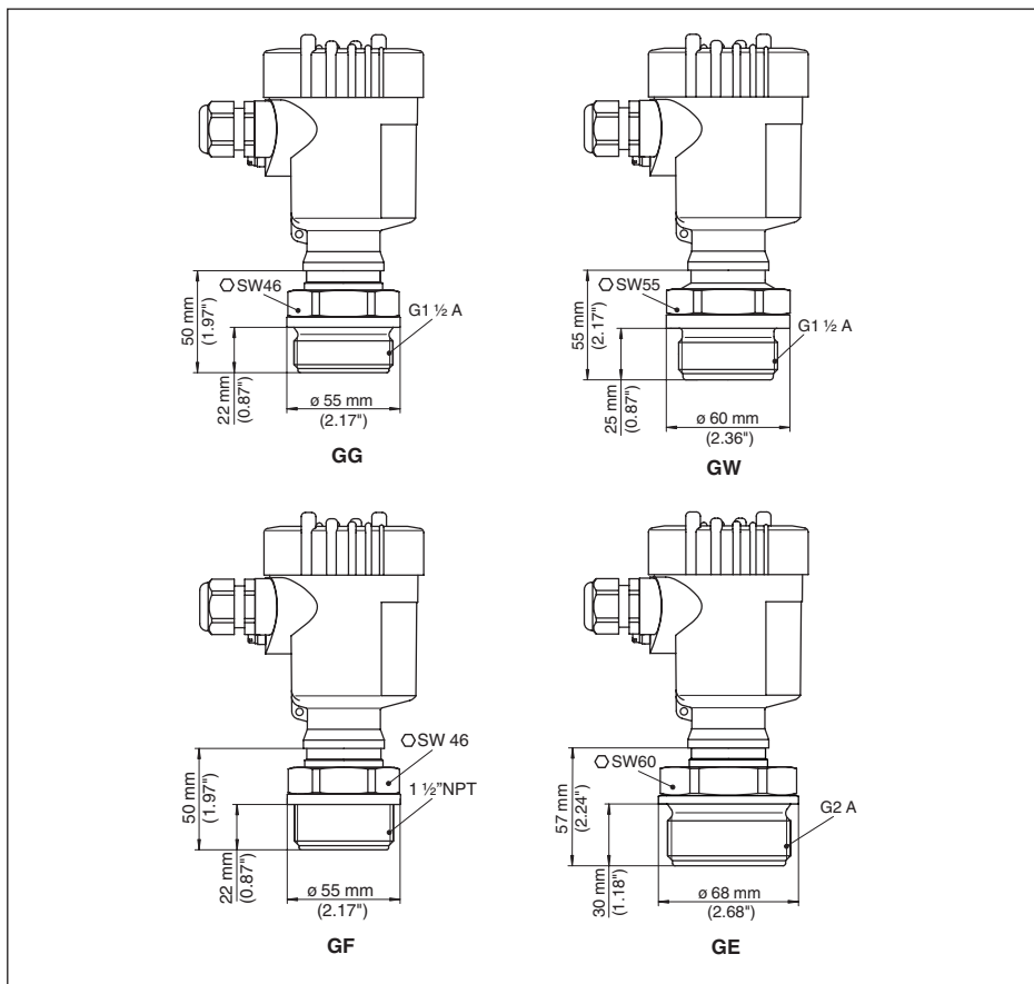
插图. 43: VEGABAR 52, 螺纹接头: GG = G1½ A, GW = G1½ A PVDF, GN = 1½ NPT, GE = G2 A
