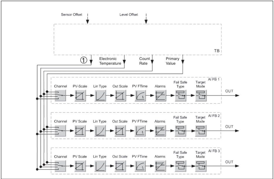
插图. 26: SOLITRAC 31: Block diagram with AI FB 1 ... AI FB 3 OUT values
