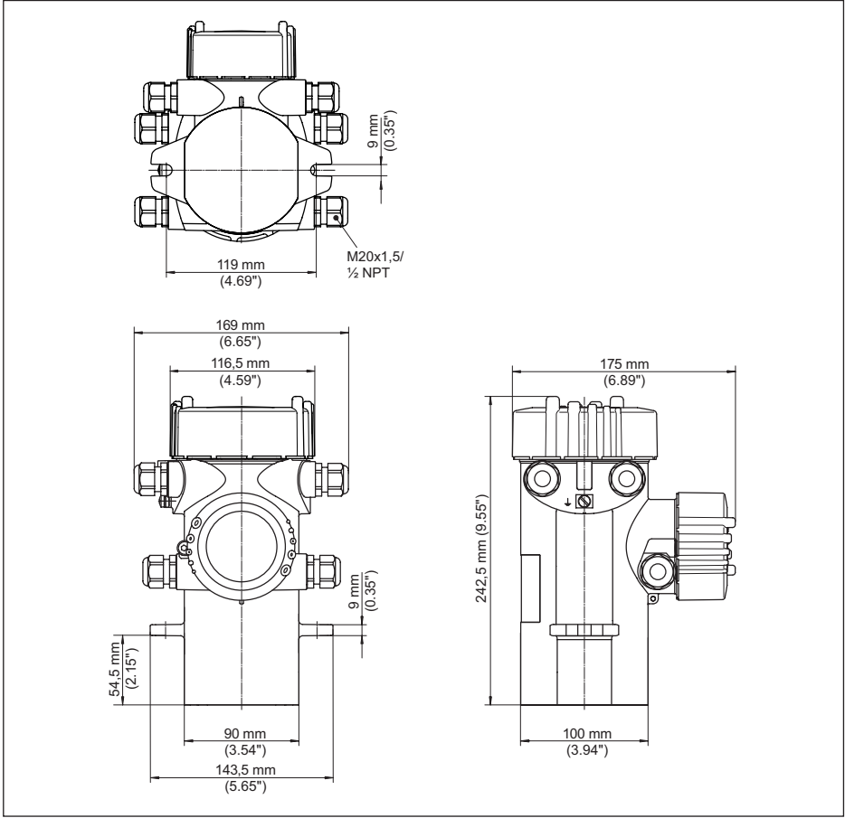
插图. 25: 铝外壳或不锈钢外壳 (精铸)
