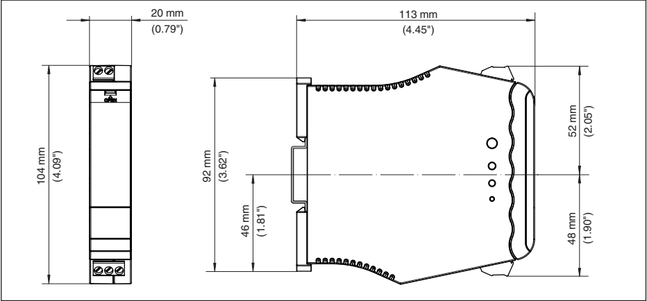
Fig. 2: Dimensions VEGATRENN 151
