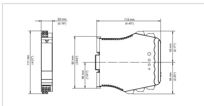
Dimensions VEGATOR 112
