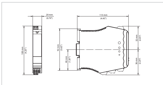
Dimensions VEGATOR 111
