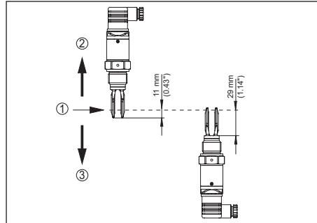
Abb. 12: Vertical mounting
