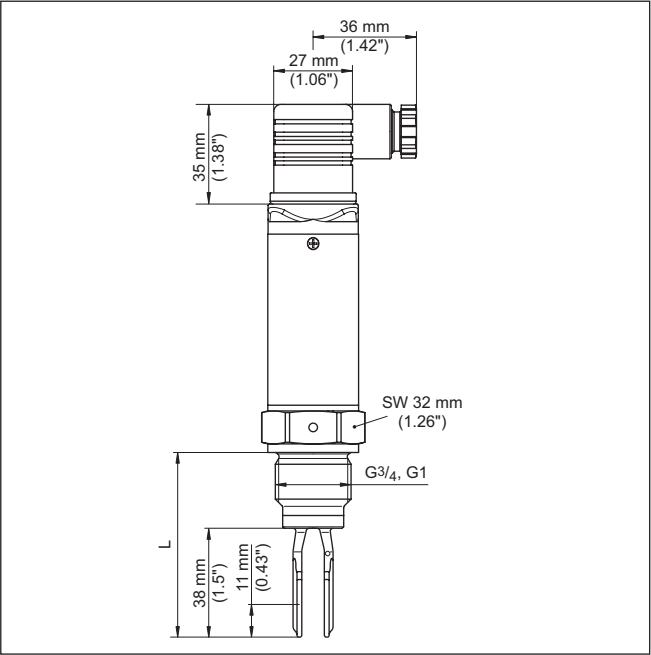
Abb. 22: VEGASWING S51 high temperature version with valve plug acc. to ISO 4400
