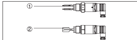
Abb. 13: Horizontal mounting
