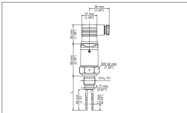
Abb. 21: VEGASWING S51 with valve block according to ISO 4400
