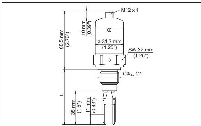
Abb. 20: VEGASWING S51 with M12 x 1 plug connection
