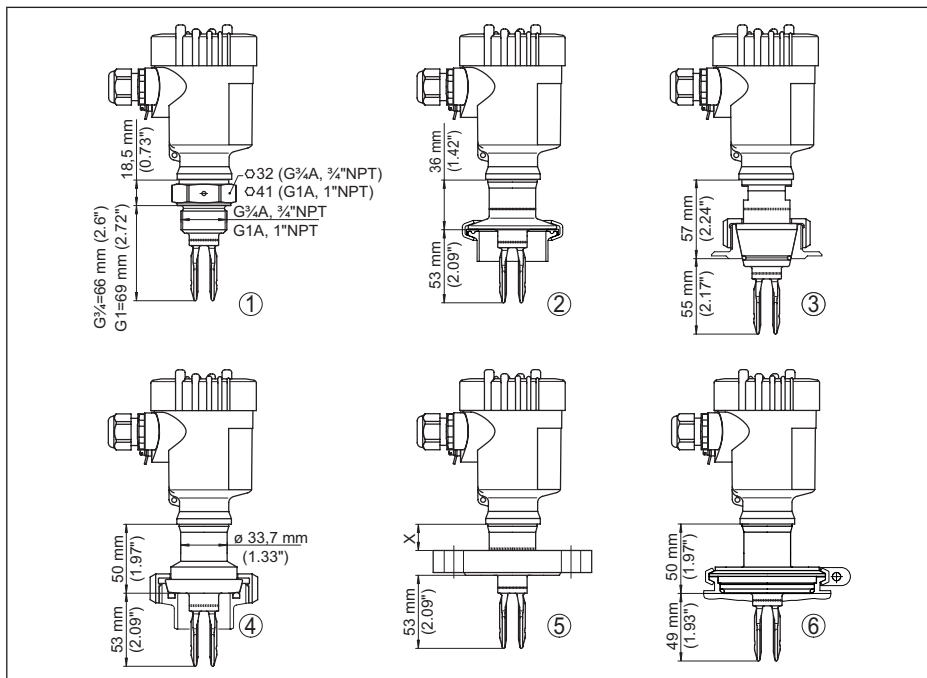
Fig. 20: VEGASWING 61
