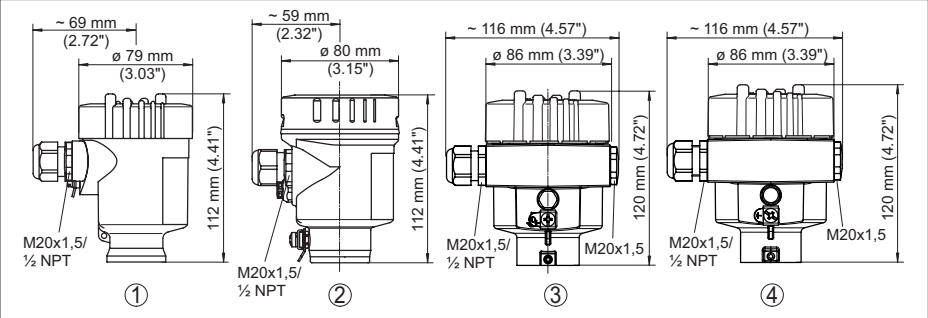
Fig. 17: Housing versions
