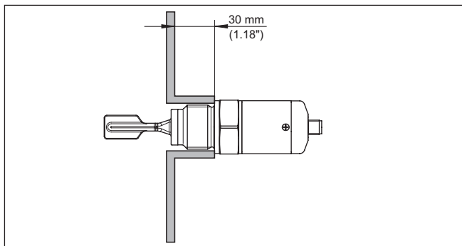
Fig. 6: Adhesive products
