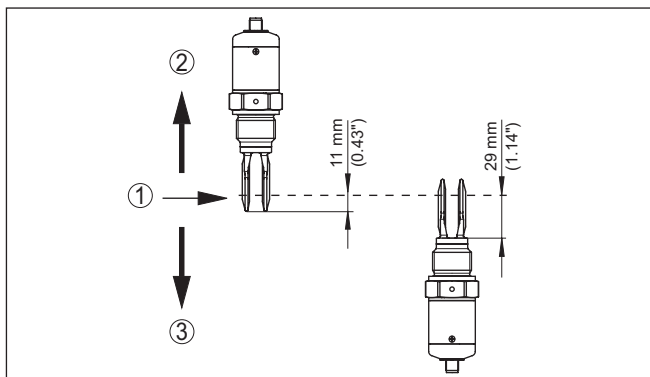
Fig. 2: Vertical mounting
