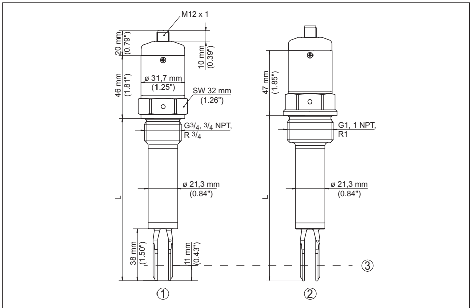
Fig. 13: VEGASWING 53, standard version, threaded fittings
