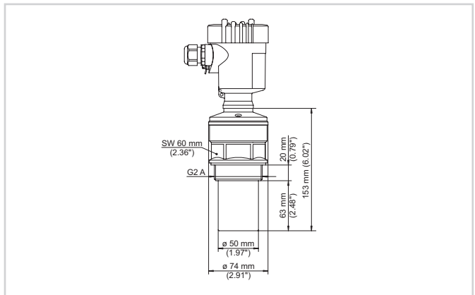
Dimensions VEGASON 62
