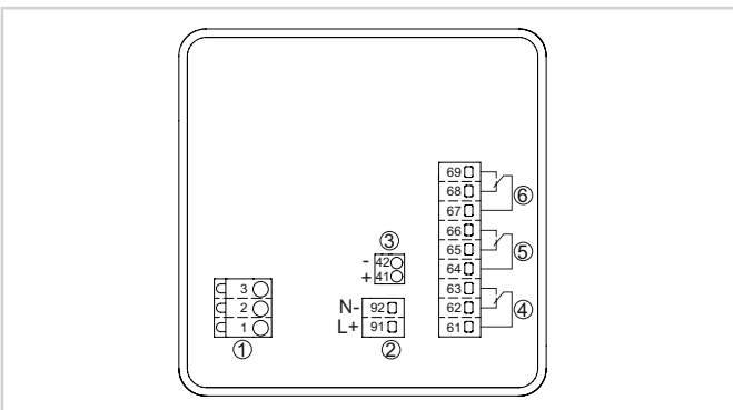
Wiring plan VEGAMET 341
