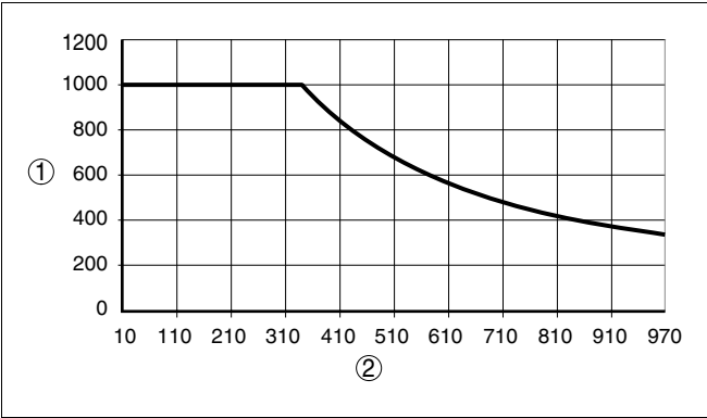
Fig. 4: Cable length in non-Ex area 1 Max. cable length in m 2 Current consumption of all connected sensors in mA
