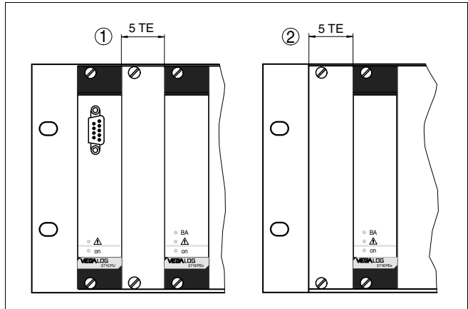
Fig. 1: Min. distances with Ex version
