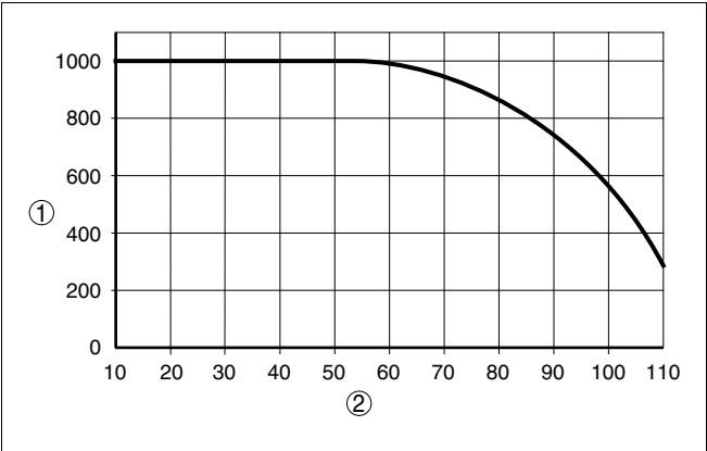
Fig. 5: Cable length in Ex area 1 Max. cable length in m 2 Current consumption of all connected sensors in mA
