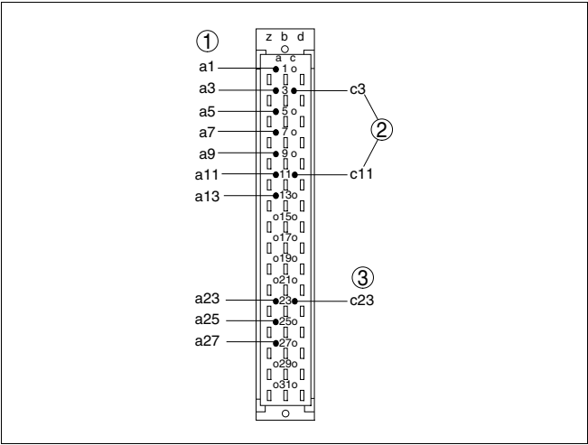
Fig. 2: Positioning of the coded pins on the male multipoint connector 1 Instrument coding 2 Function coding 3 Ex coding
