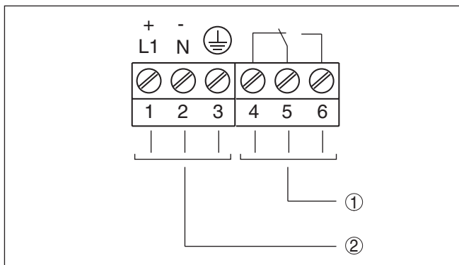
Fig. 4: Electronics with relay output
