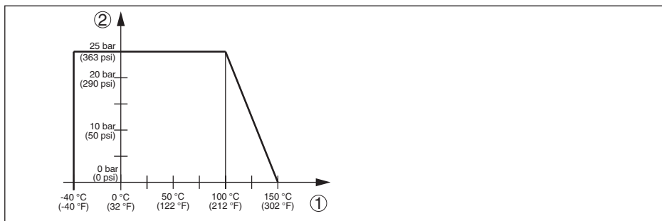
Fig. 6: Process temperature - Process pressure
