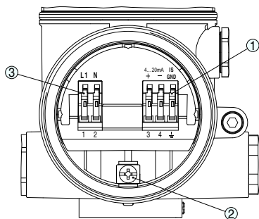
Connection compartment double chamber housing
