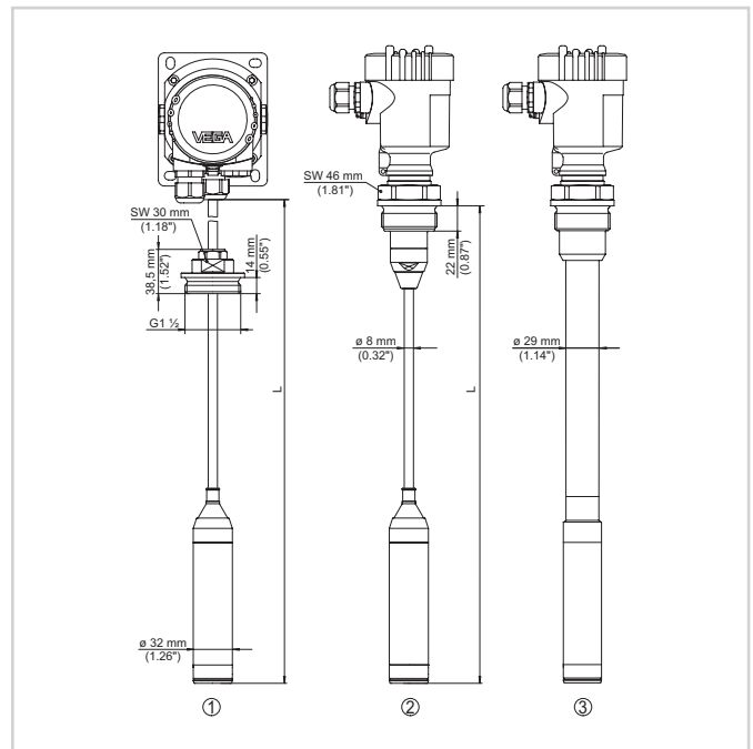
Dimensions VEGABAR 66
