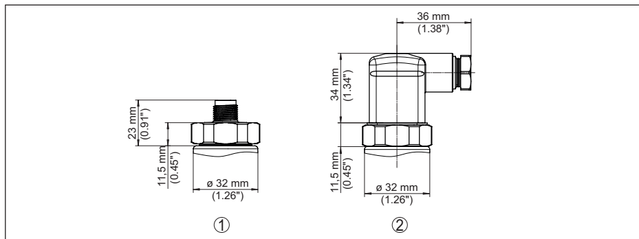
Fig. 15: VEGABAR 18 housing
