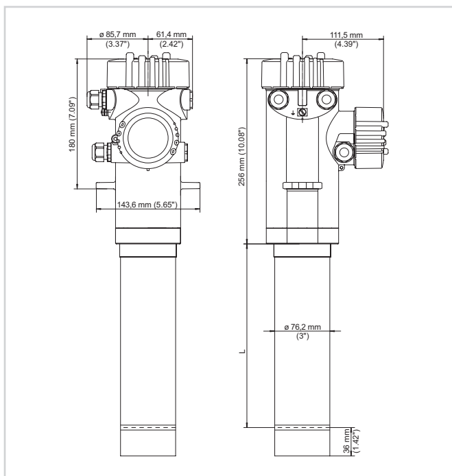
Dimensions SOLITRAC 31
