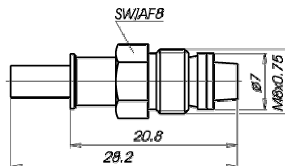
Figure 9: Recommended antenna connector
