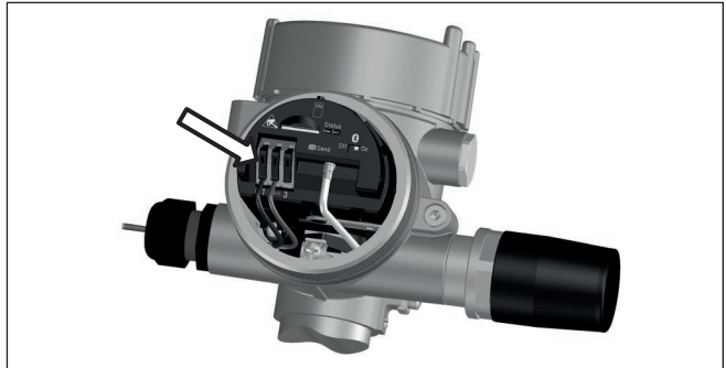
Fig. 2: Connection steps 4 and 5
