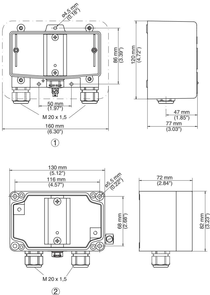
Fig. 11: Dimensions B62-30W
