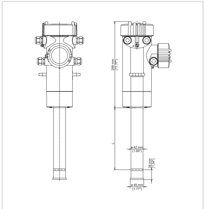
Dimensions FIBERTRAC 31
