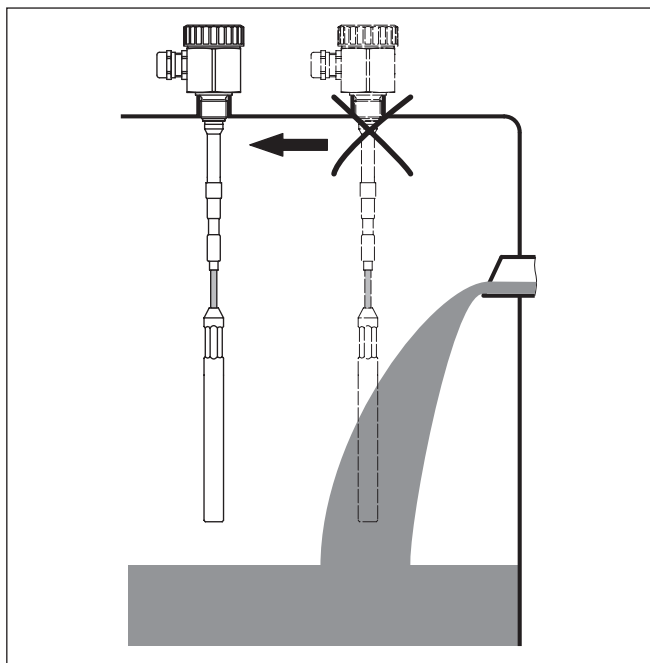
Fig. 2: Inflowing medium
