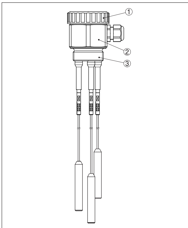
Fig. 1: Conductive multiple cable electrode EL 5
