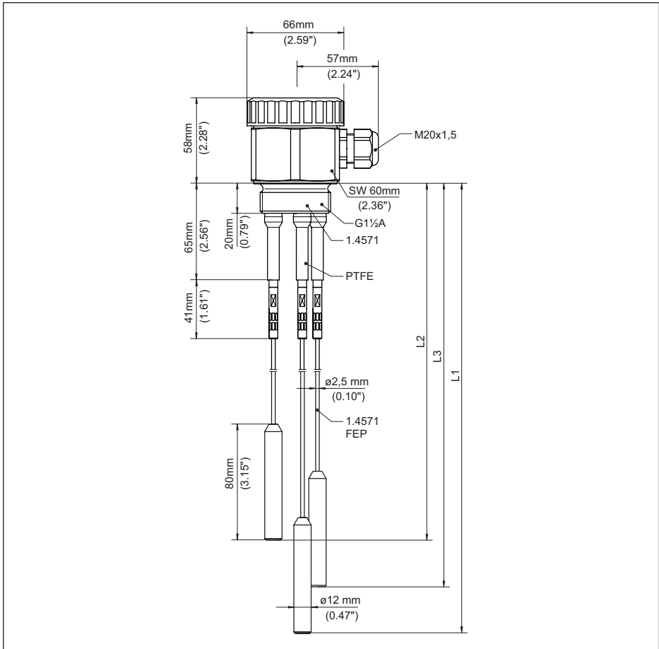
Fig. 6: Conductive multiple cable electrode EL 5
