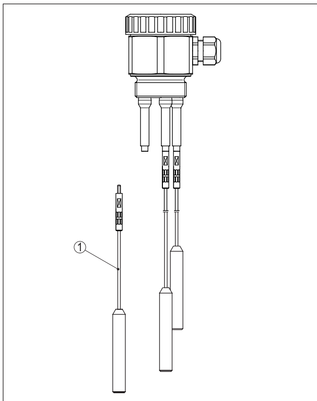
Fig. 5: Insertion of a cable electrode
