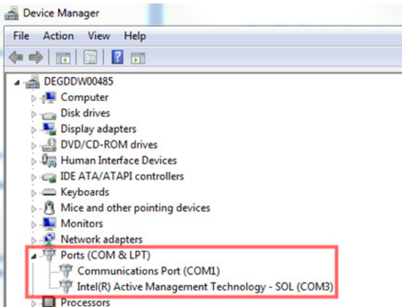
图 47: Device Manager
