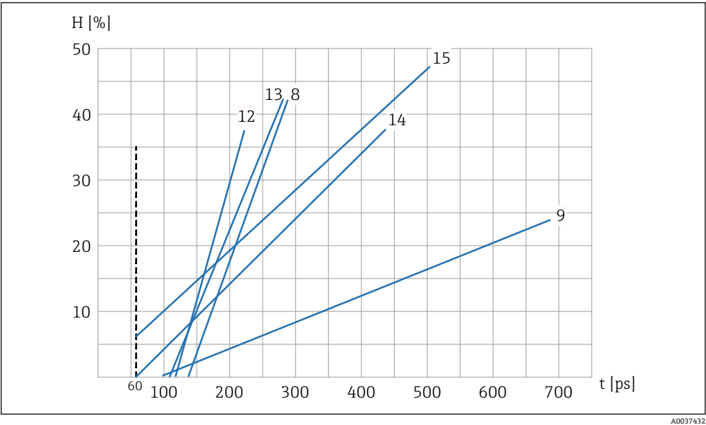
图 20 标定曲线集 A (Cal.8, Cal.9, Cal.12, Cal.13, Cal.14, Cal.15)
