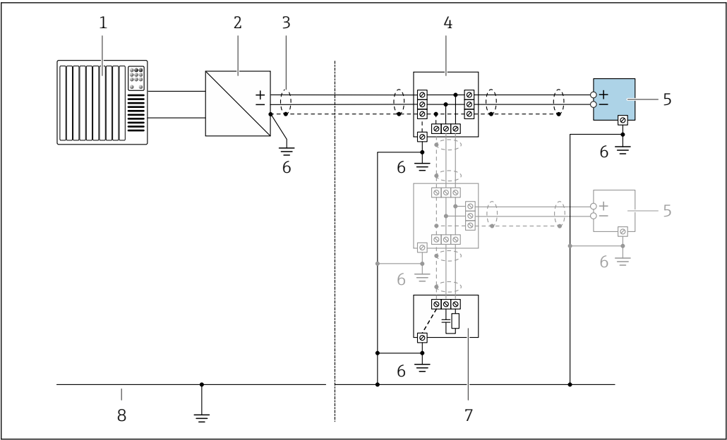
12 接线实例：FOUNDATION Fieldbus
